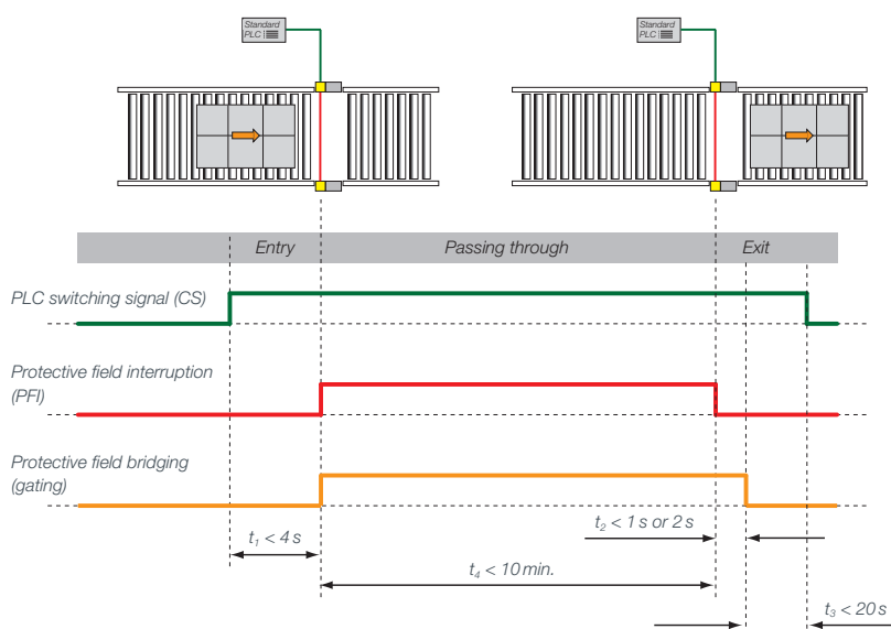
Figure 4: Signal progress whilst transport material is passing through the protective field
