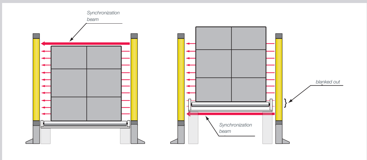
Figure 9: Use of the top or bottom beam as synchronization beam
