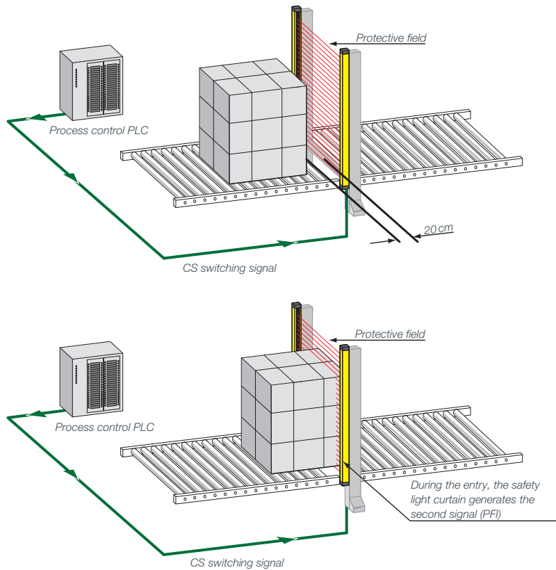
Figure 3: Overview of the operating principle
